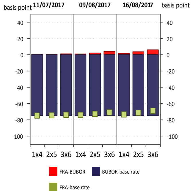
84. Difference between the 3 month FRA quotes and the current base rate
