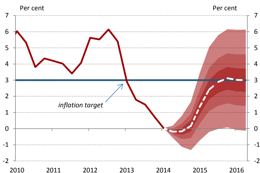
Annual inflation projection fan chart
