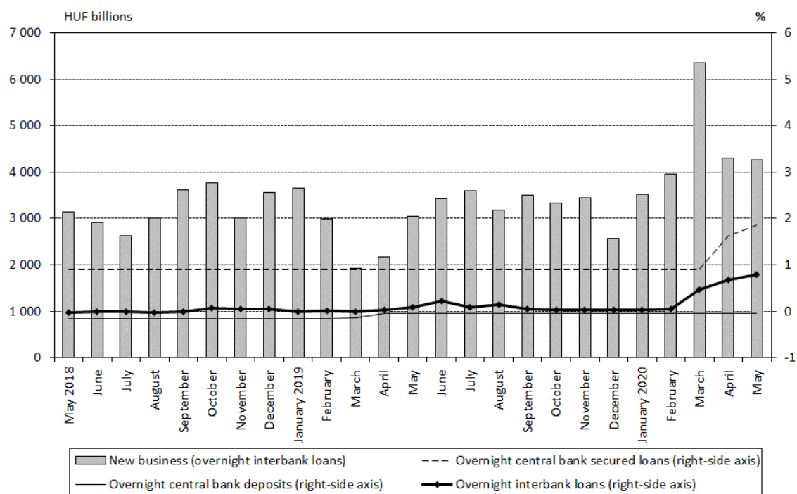
Chart 13 Average overnight interbank rates, total interbank lending and the interest rate corridor
