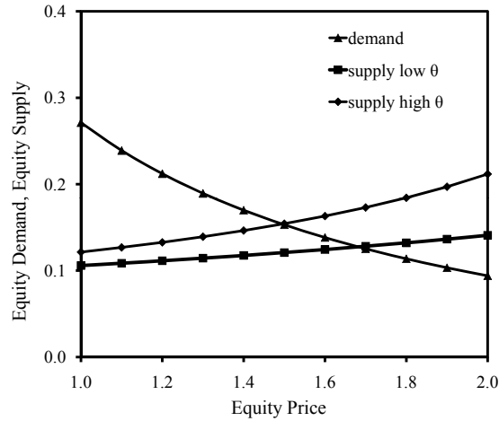
Figure 4.2: Demand and supply of equity for various levels of \theta
