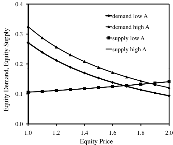
Figure 4.3: Demand and supply of equity for various levels of A
