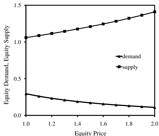
Figure 4.4: Demand and supply of equity as a function of the price of equity
