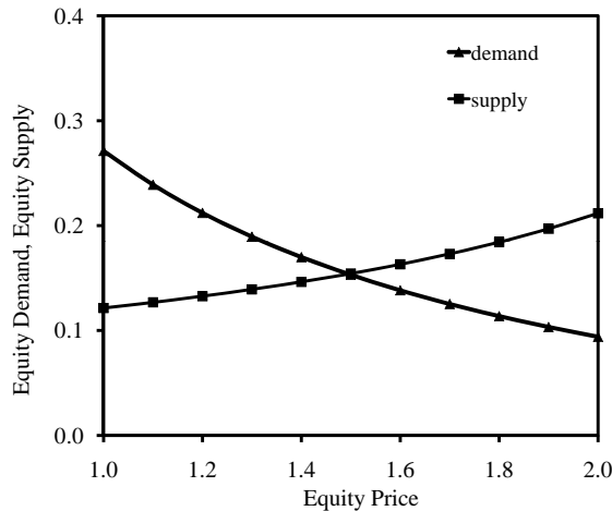
Figure 4.1: Demand and supply of equity as a function of the price of equity
