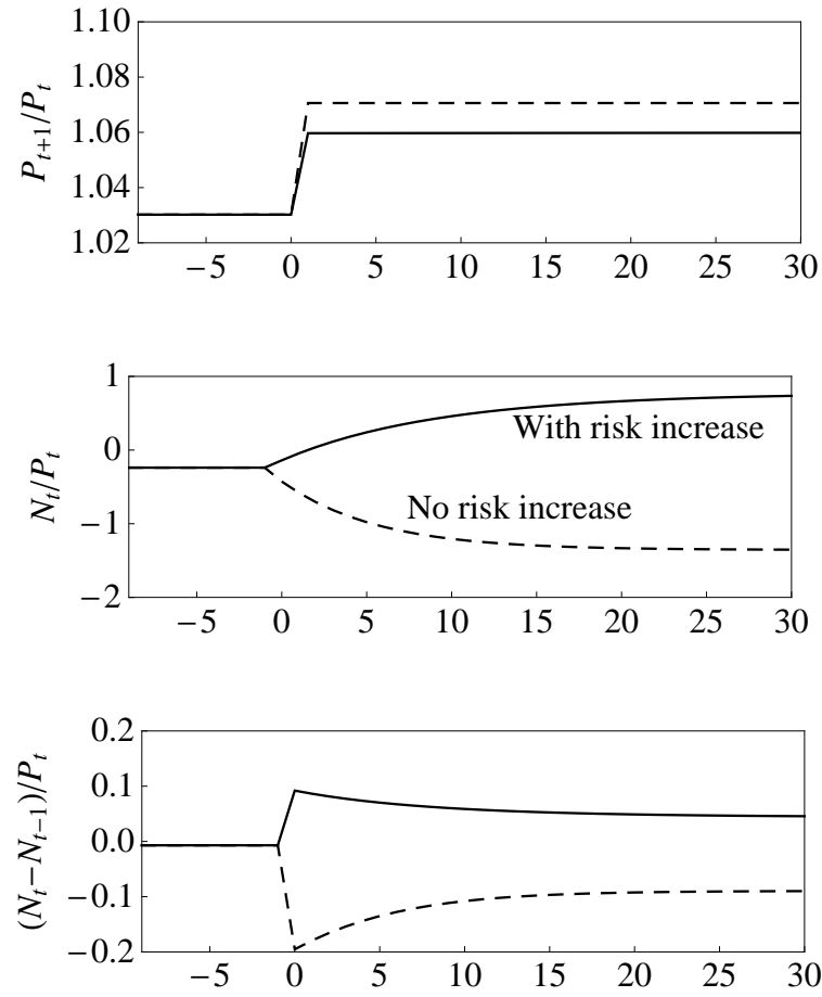
Figure 5 Transition Dynamics
