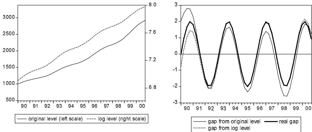
Figure 4 Distortion in HP filtered exponential time series
